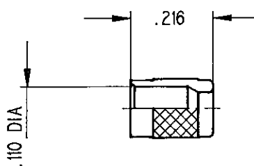
INTERMEDIATE FERRULE
