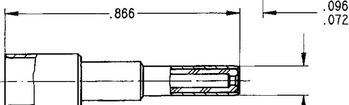
INTERMEDIATE CONTACT
